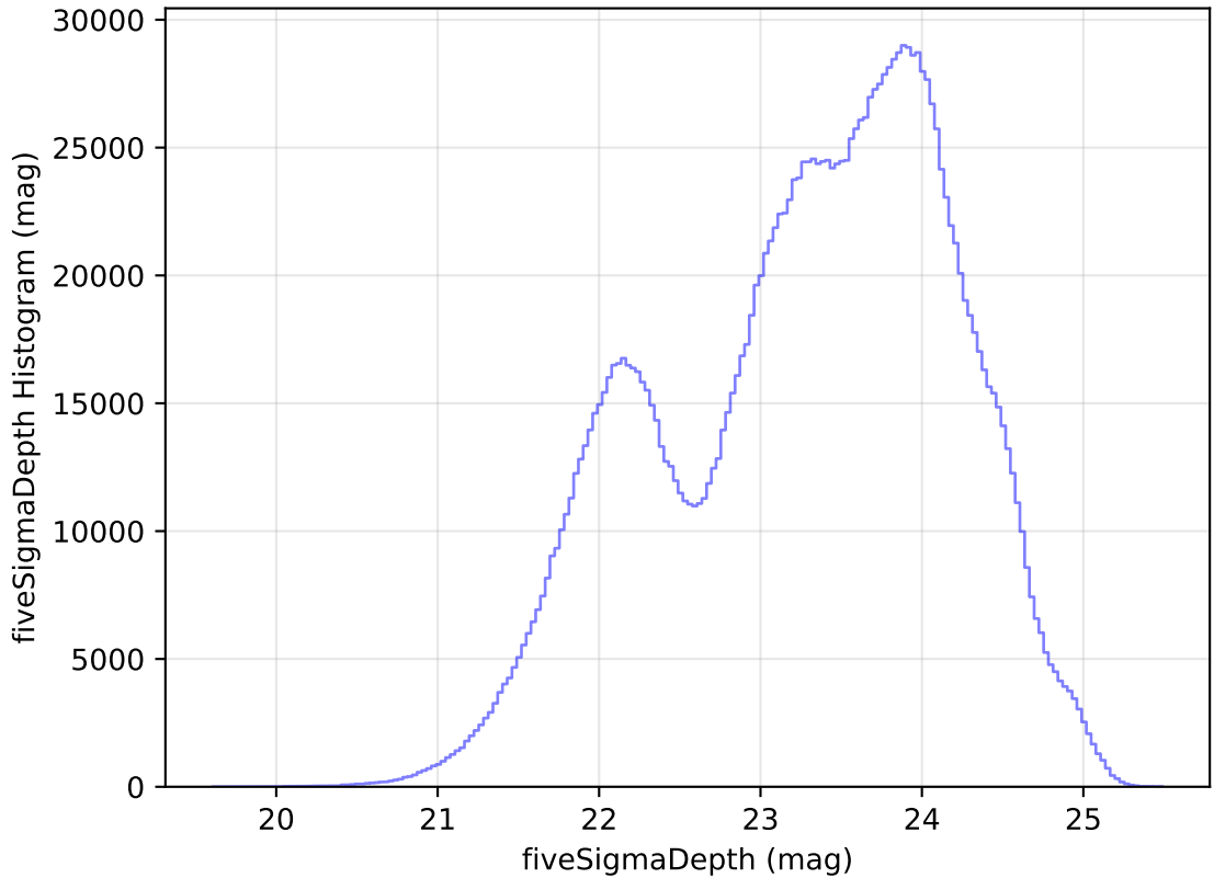
internal_u_expt60_nscale1.1v3.4_10yrs All sky all bands: fiveSigmaDepth Histogram
