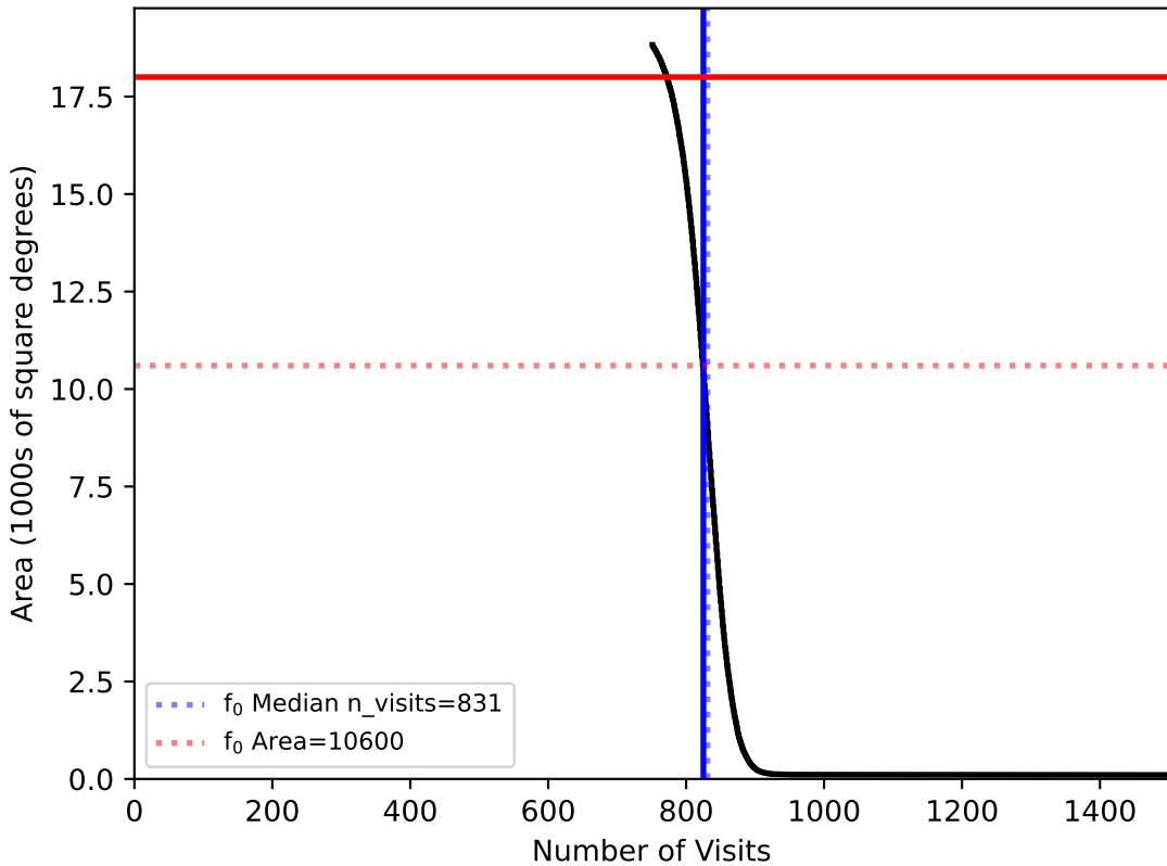
internal_u_expt60_nscale1.1v3.4_10yrs WFD: fO
