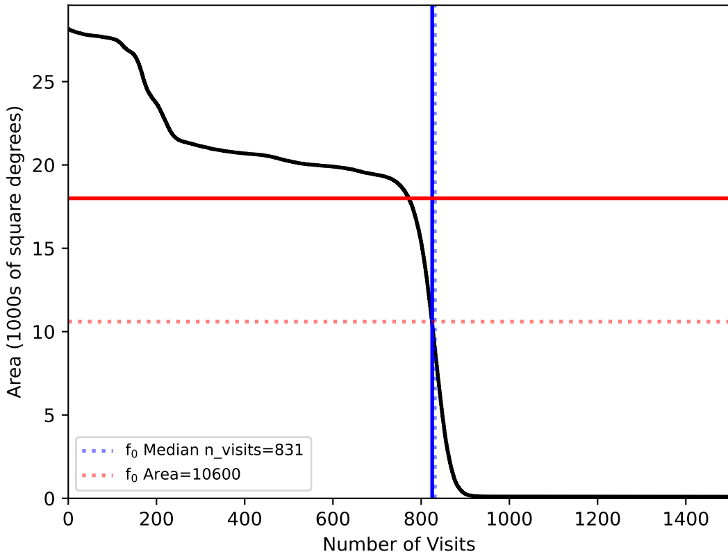
internal_u_expt60_nscale1.1v3.4_10yrs All sky: f0
