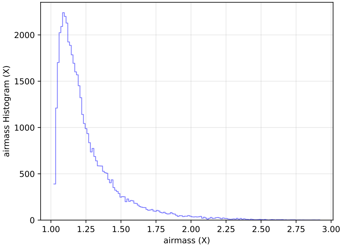
internal_u_expt60_nscale1.1v3.4_10yrs Yr 1 y band: airmass Histogram
