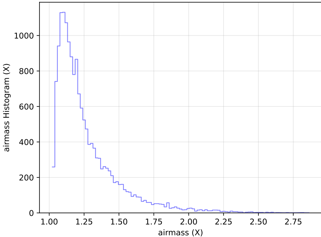
internal_u_expt60_nscale1.1v3.4_10yrs Yr 1 u band: airmass Histogram
