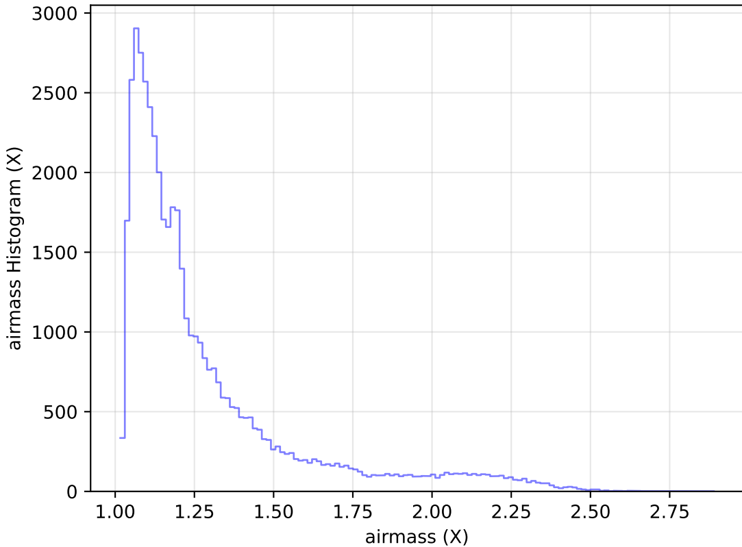
internal_u_expt60_nscale1.1v3.4_10yrs Yr 1 r band: airmass Histogram
