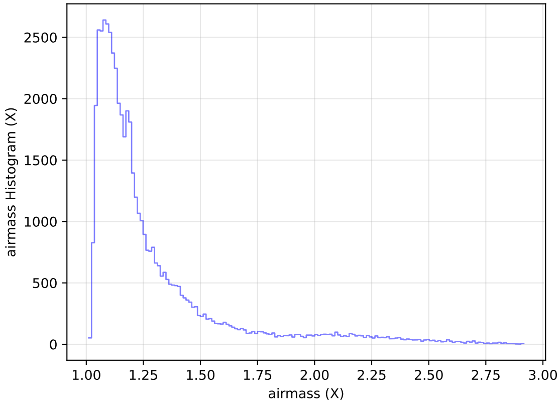
internal_u_expt60_nscale1.1v3.4_10yrs Yr 1 i band: airmass Histogram
