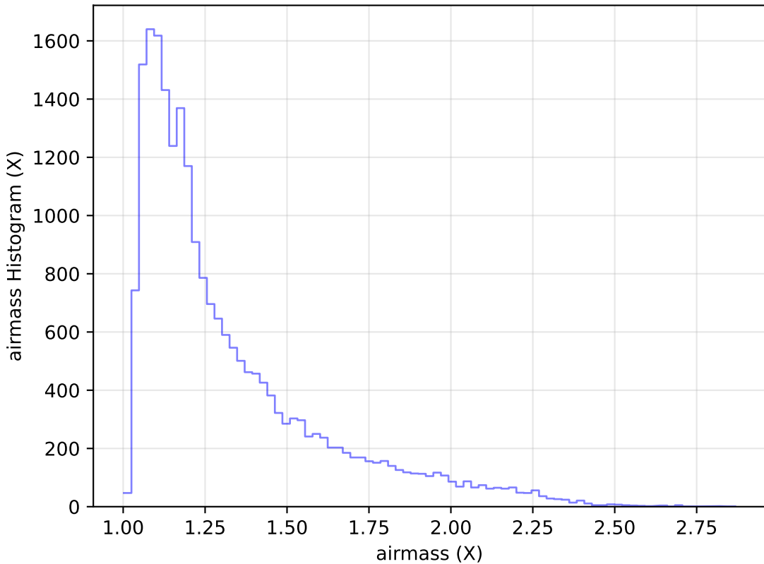
internal_u_expt60_nscale1.1v3.4_10yrs Yr 1 g band: airmass Histogram
