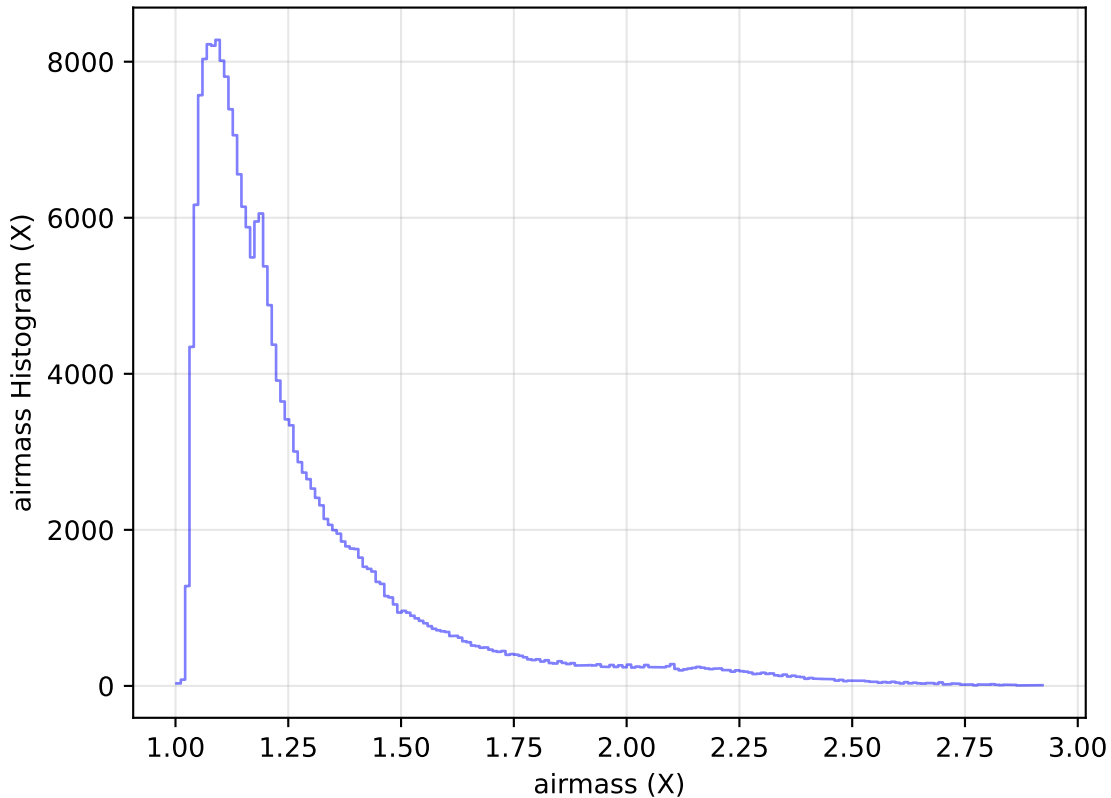
internal_u_expt60_nscale1.1v3.4_10yrs Yr 1 all bands: airmass Histogram
