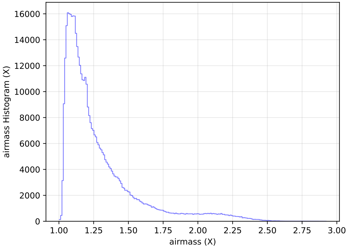
internal_u_expt60_nscale1.1v3.4_10yrs WFD r band: airmass Histogram
