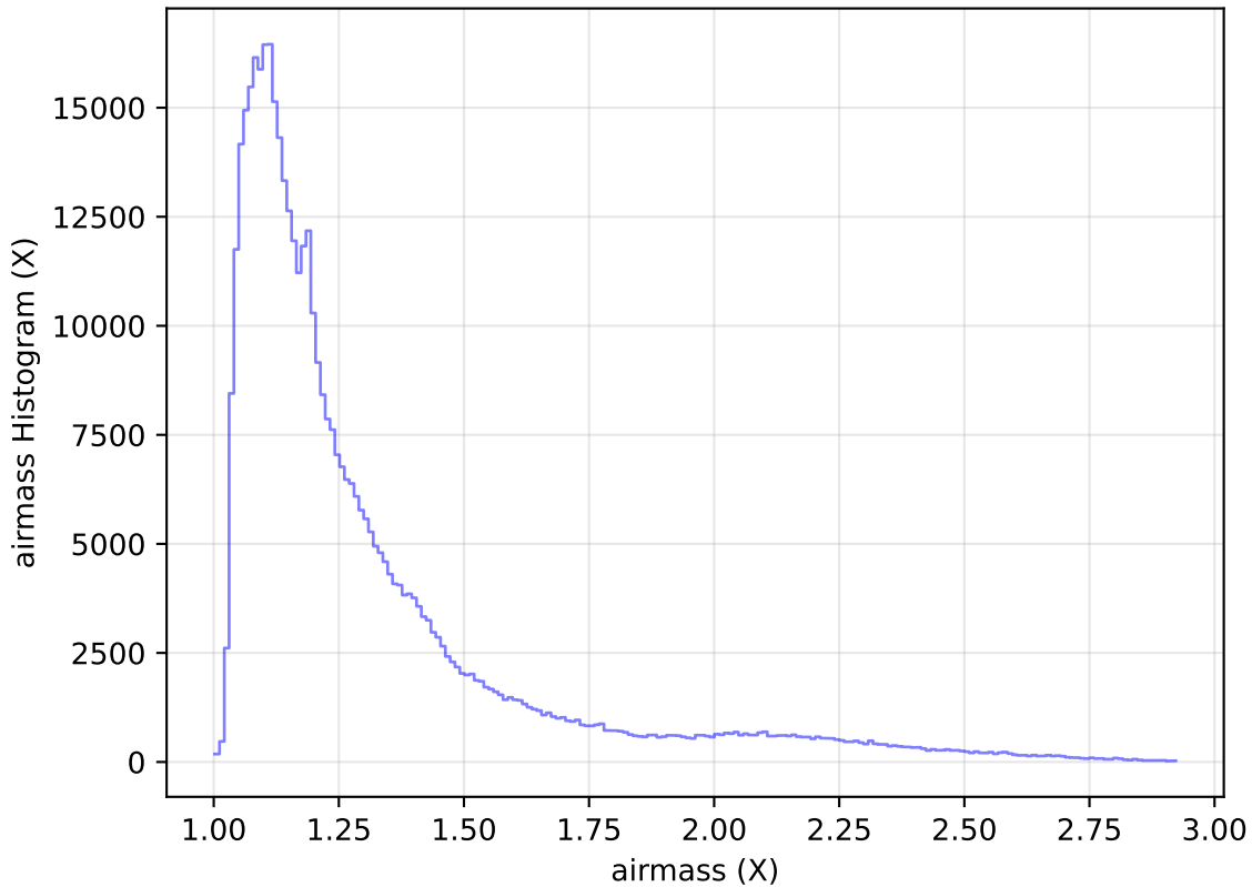
internal_u_expt60_nscale1.1v3.4_10yrs WFD i band: airmass Histogram
