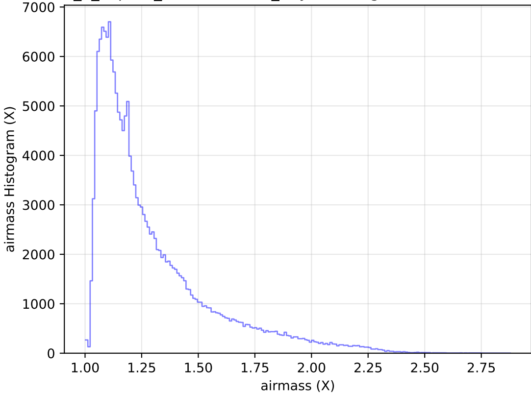
internal_u_expt60_nscale1.1v3.4_10yrs WFD g band: airmass Histogram
