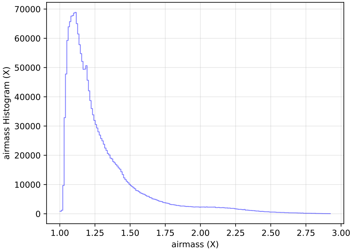
internal_u_expt60_nscale1.1v3.4_10yrs WFD all bands: airmass Histogram
