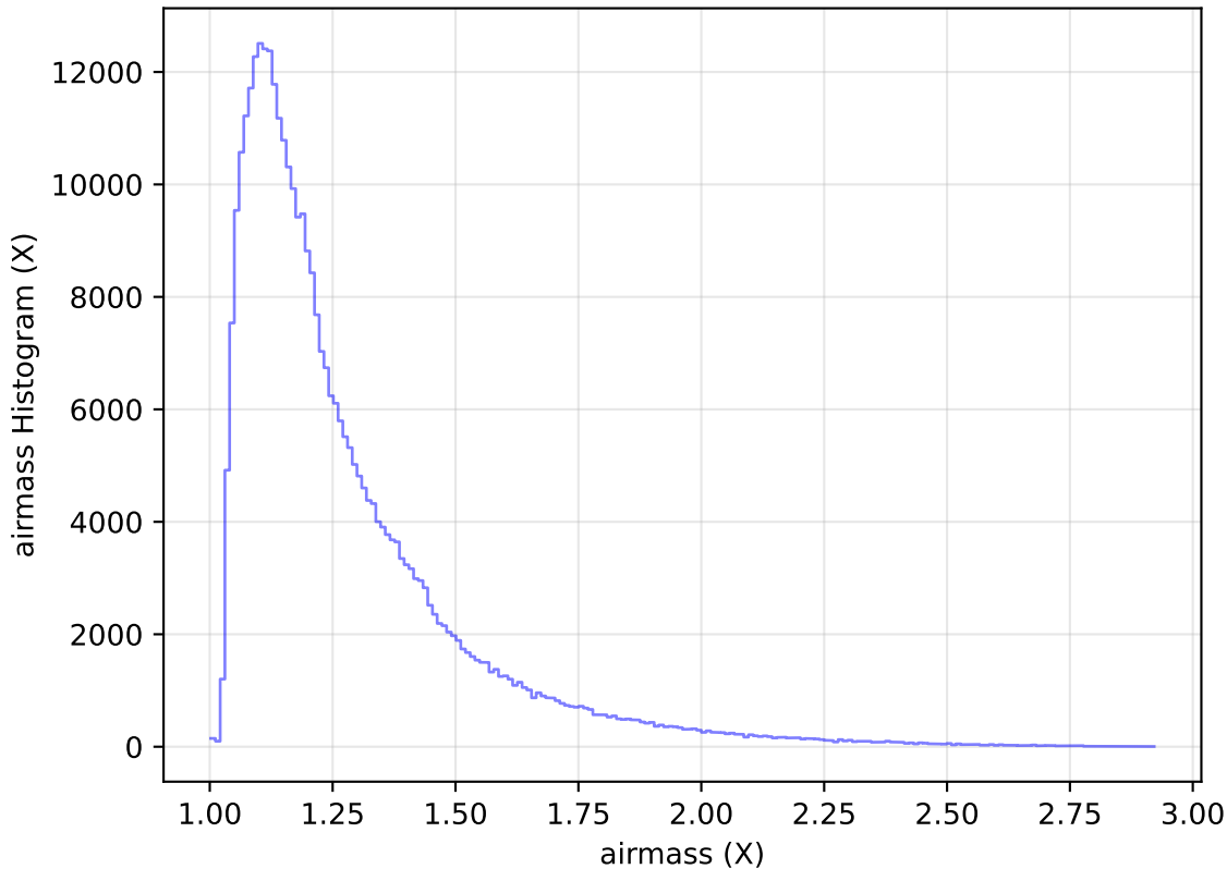
internal_u_expt60_nscale1.1v3.4_10yrs All sky y band: airmass Histogram
