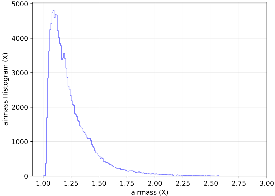
internal_u_expt60_nscale1.1v3.4_10yrs All sky u band: airmass Histogram
