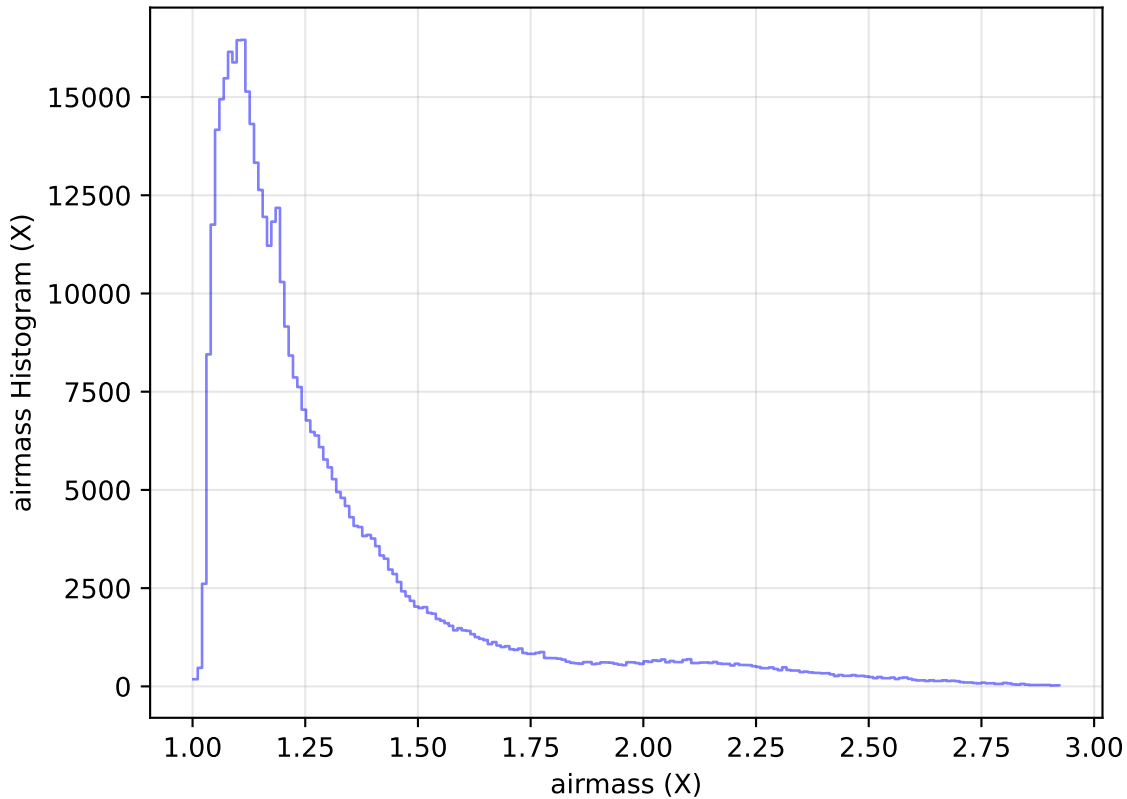
internal_u_expt60_nscale1.1v3.4_10yrs All sky i band: airmass Histogram
