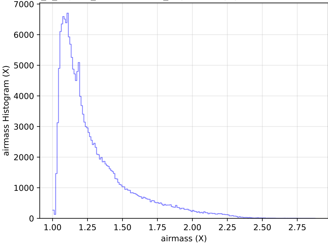
internal_u_expt60_nscale1.1v3.4_10yrs All sky g band: airmass Histogram
