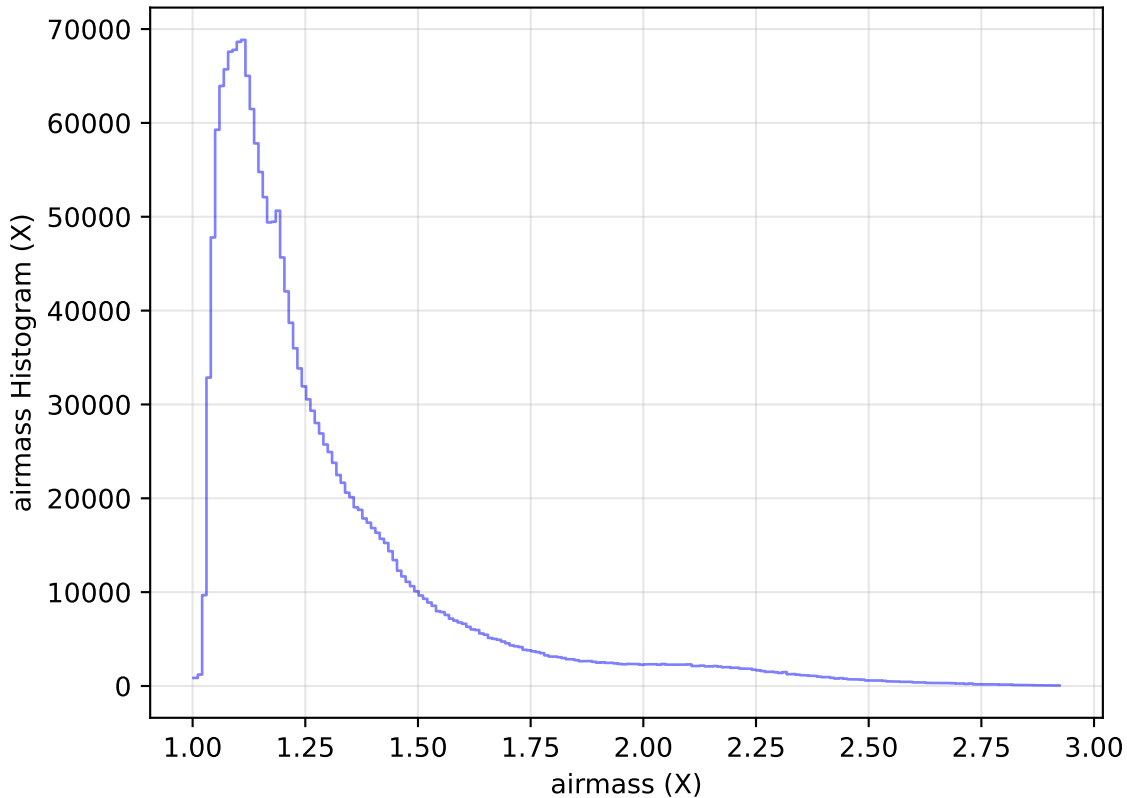
internal_u_expt60_nscale1.1v3.4_10yrs All sky all bands: airmass Histogram
