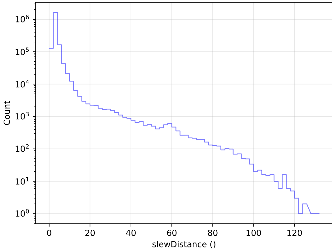
internal_u_expt60_nscale1.1v3.4_10yrs All visits: Slew Distance Histogram
