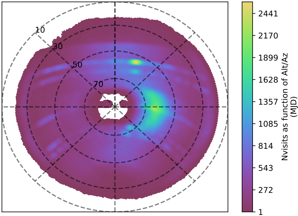
internal_u_expt60_nscale1.1v3.4_10yrs z band: Nvisits as function of Alt/Az
