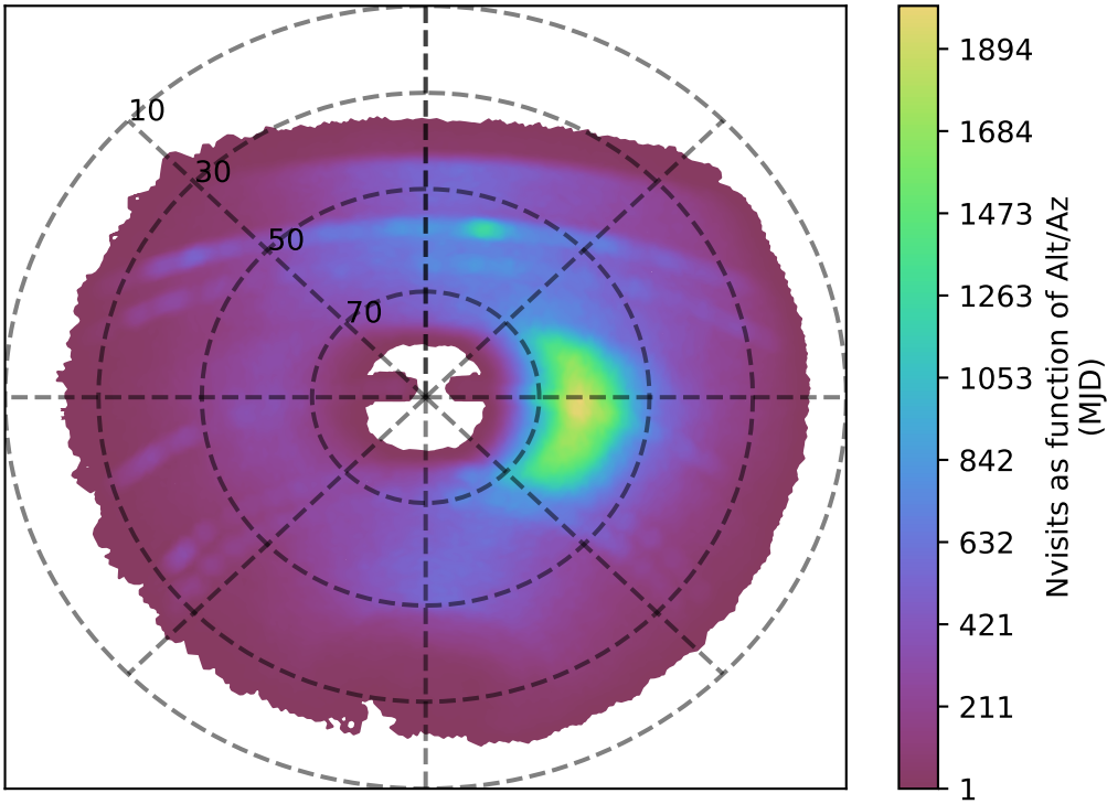
internal_u_expt60_nscale1.1v3.4_10yrs y band: Nvisits as function of Alt/Az
