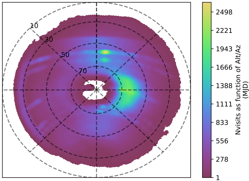
internal_u_expt60_nscale1.1v3.4_10yrs r band: Nvisits as function of Alt/Az
