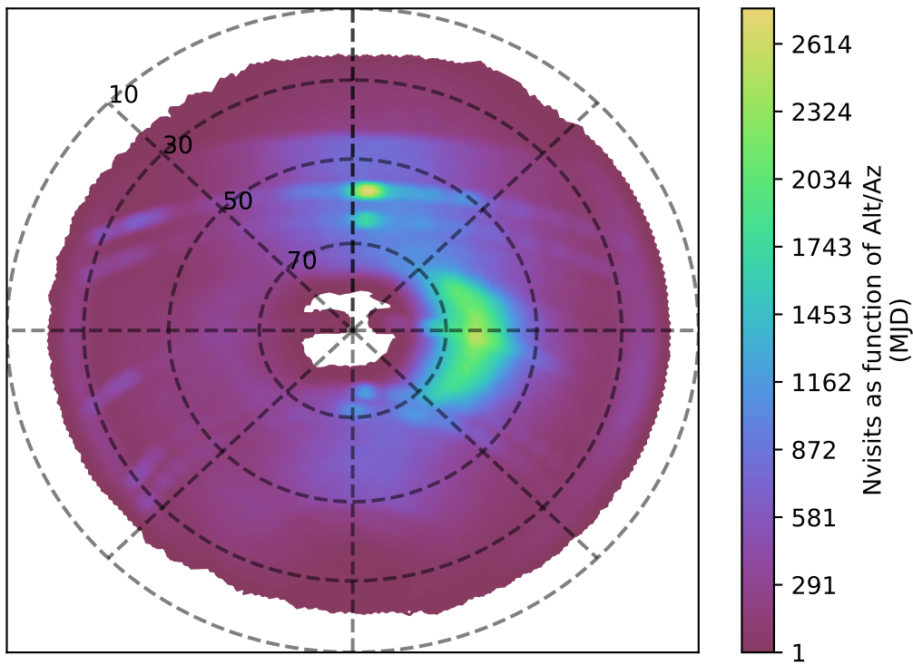
internal_u_expt60_nscale1.1v3.4_10yrs i band: Nvisits as function of Alt/Az
