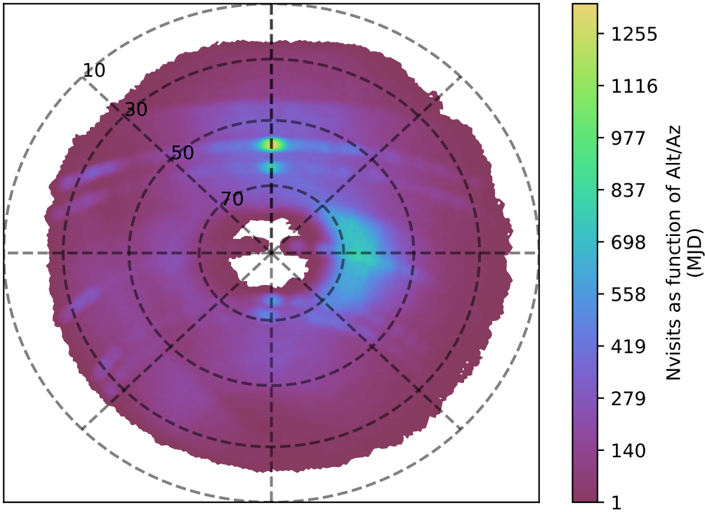
internal_u_expt60_nscale1.1v3.4_10yrs g band: Nvisits as function of Alt/Az
