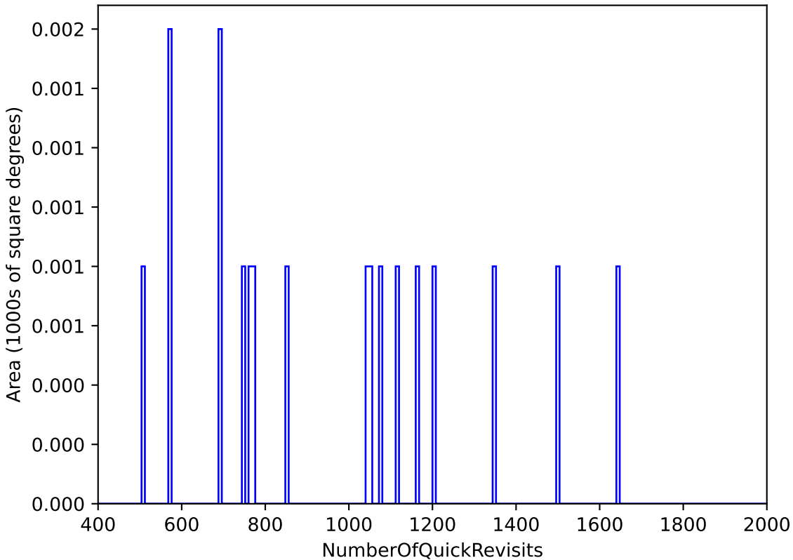
internal_u_expt60_nscale1.1v3.4_10yrs WFD: NumberOfQuickRevisits
