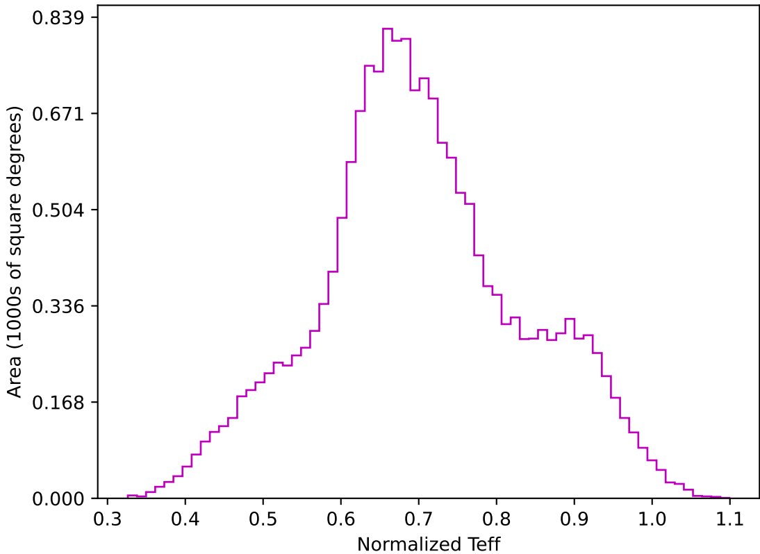
internal_u_expt60_nscale1.1v3.4_10yrs WFD z band: Normalized Teff
