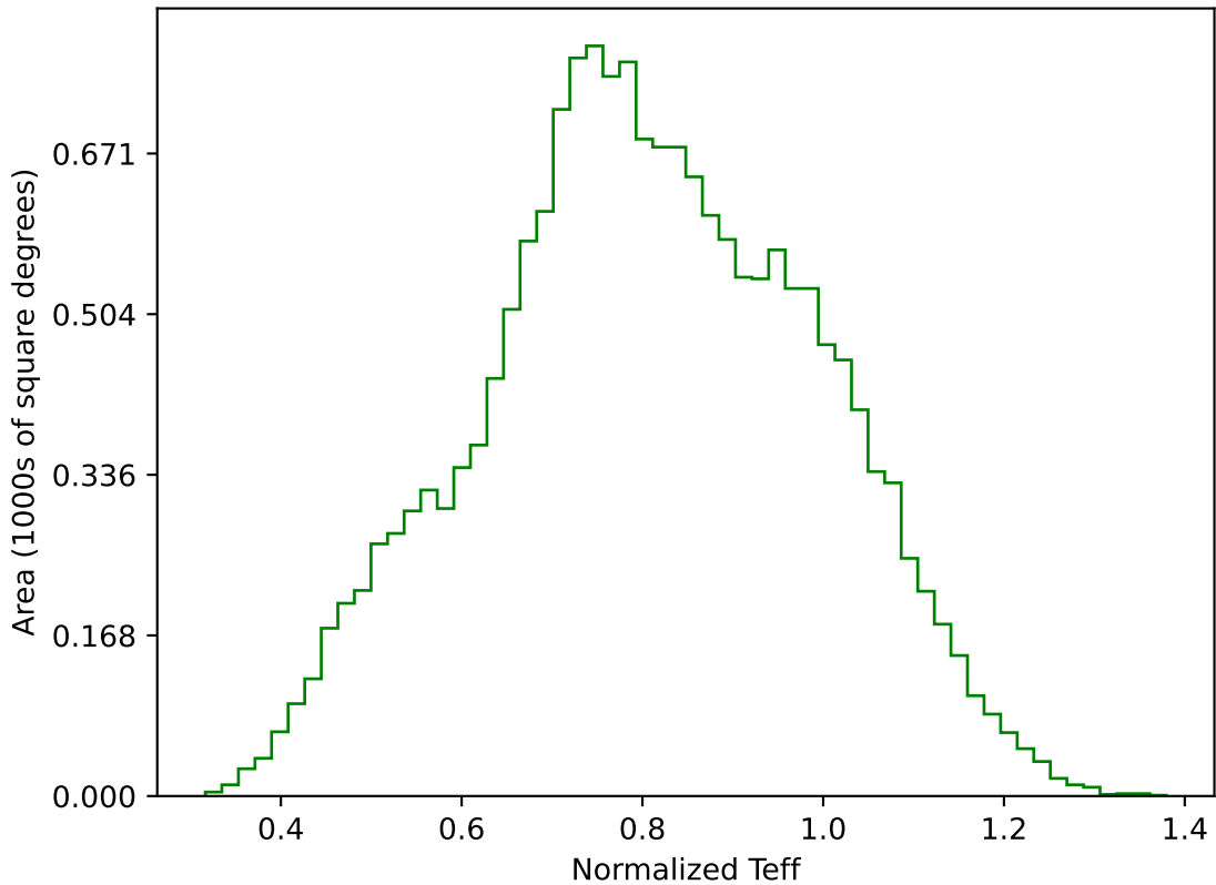
internal_u_expt60_nscale1.1v3.4_10yrs WFD g band: Normalized Teff
