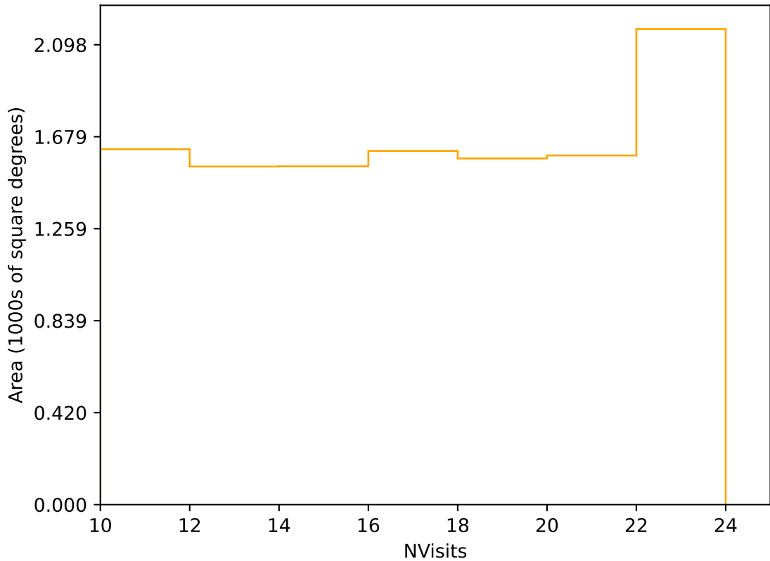
internal_u_expt60_nscale1.1v3.4_10yrs Yr 3-4 r band: NVisits
