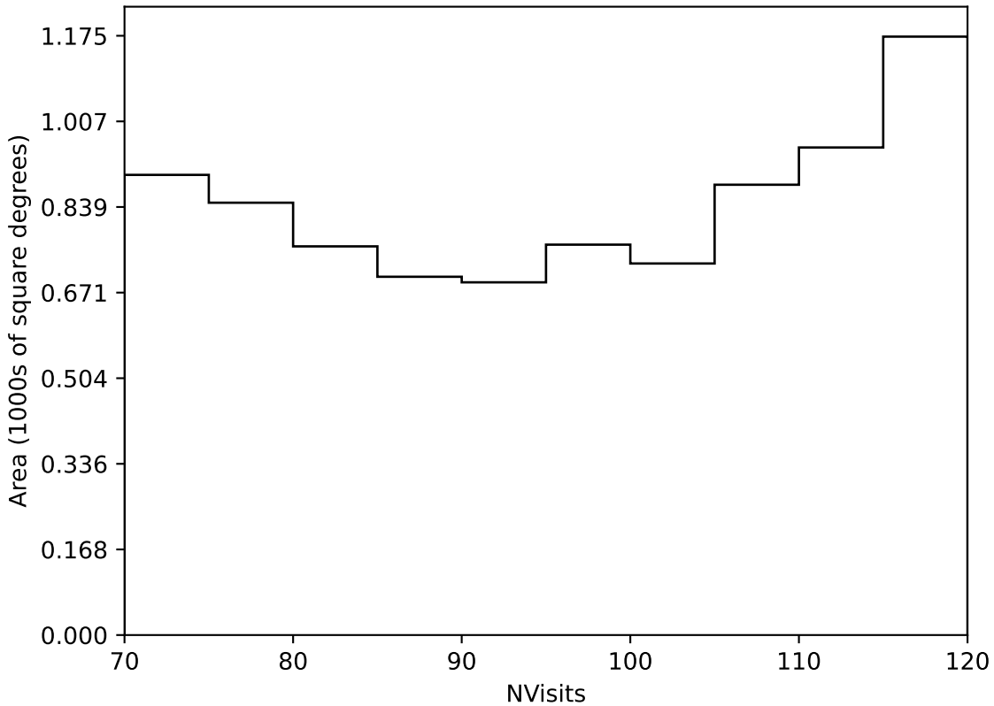
internal_u_expt60_nscale1.1v3.4_10yrs Yr 3-4 all bands: NVisits
