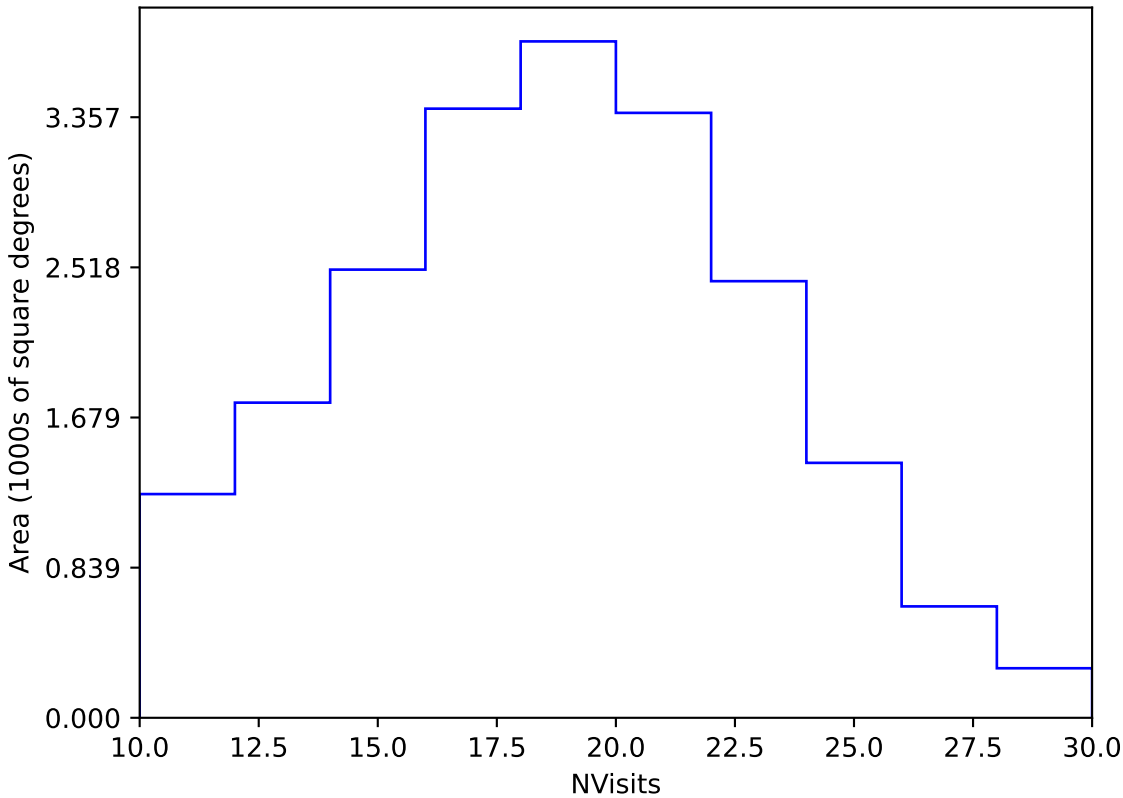
internal_u_expt60_nscale1.1v3.4_10yrs Yr 1 y band: NVisits
