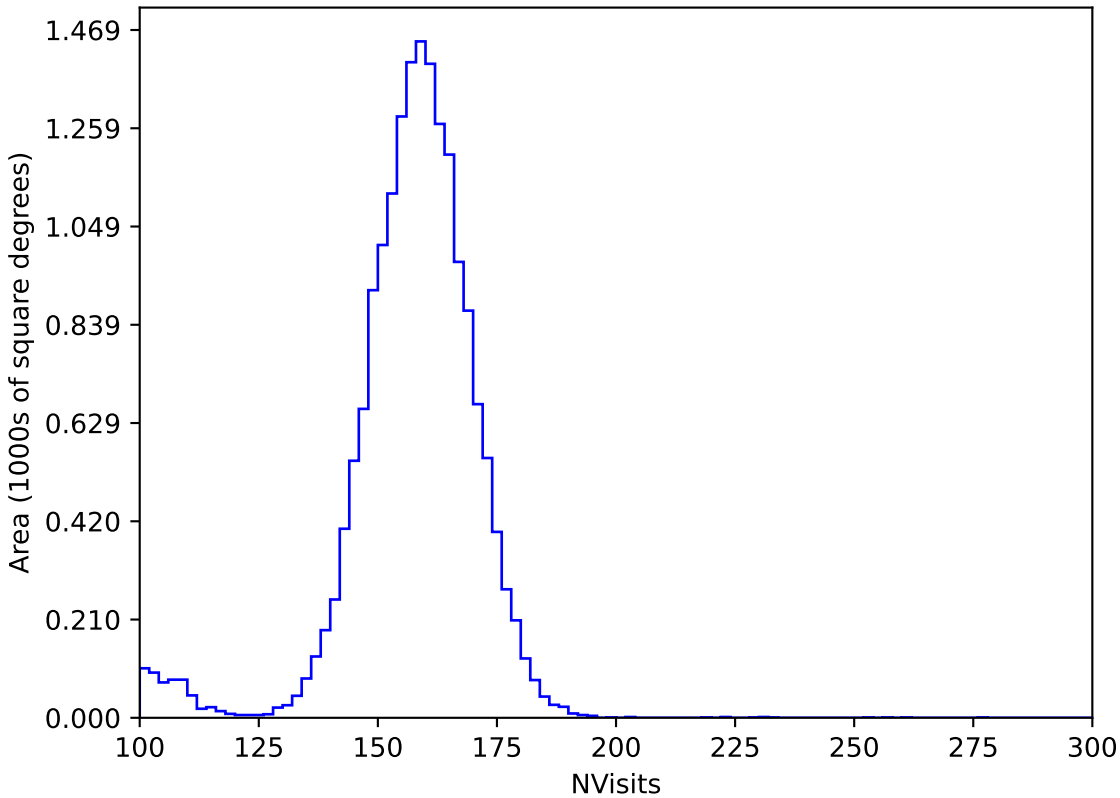
internal_u_expt60_nscale1.1v3.4_10yrs WFD y band: NVisits
