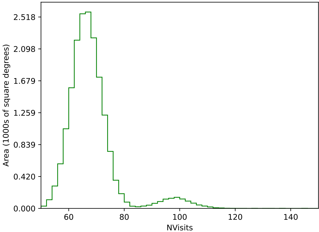
internal_u_expt60_nscale1.1v3.4_10yrs WFD g band: NVisits
