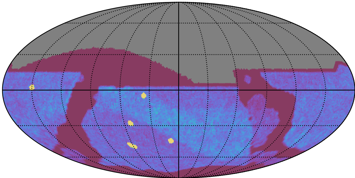
internal_u_expt60_nscale1.1v3.4_10yrs All sky z band: NVisits
