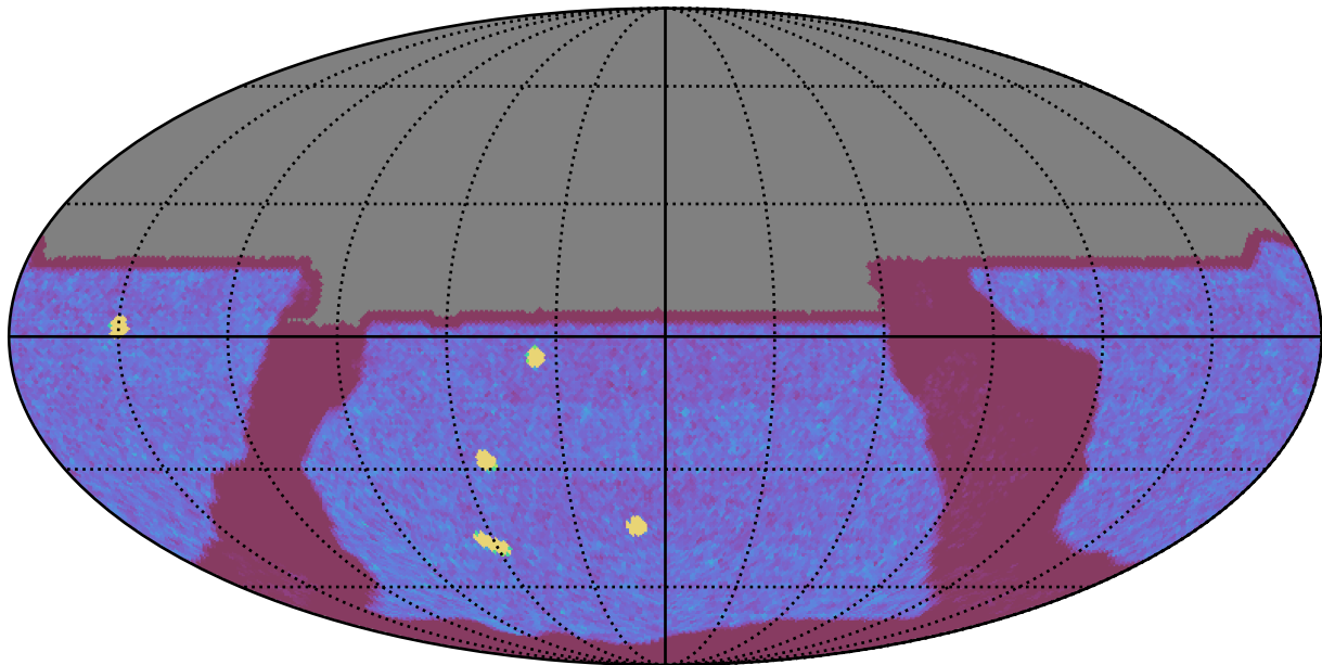
internal_u_expt60_nscale1.1v3.4_10yrs All sky y band: NVisits
