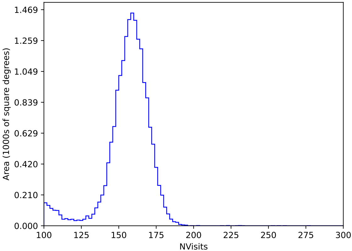
internal_u_expt60_nscale1.1v3.4_10yrs All sky y band: NVisits
