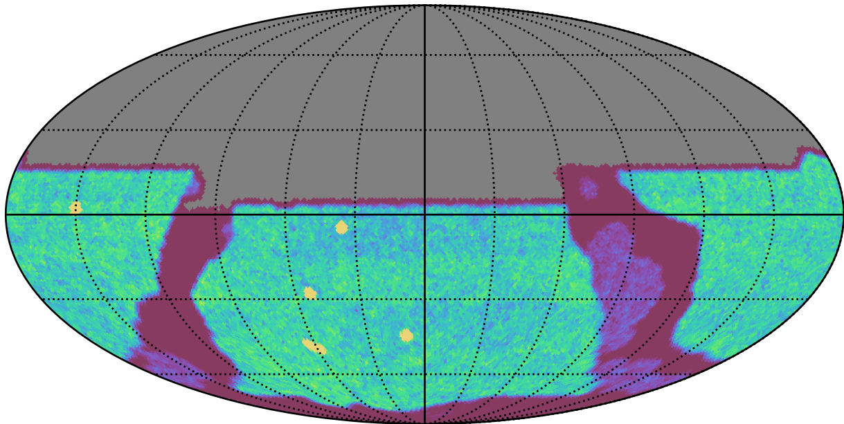
internal_u_expt60_nscale1.1v3.4_10yrs All sky u band: NVisits
