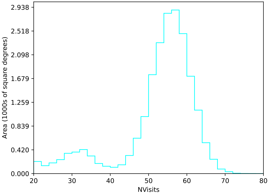
internal_u_expt60_nscale1.1v3.4_10yrs All sky u band: NVisits
