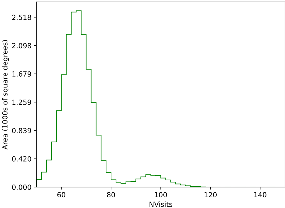
internal_u_expt60_nscale1.1v3.4_10yrs All sky g band: NVisits
