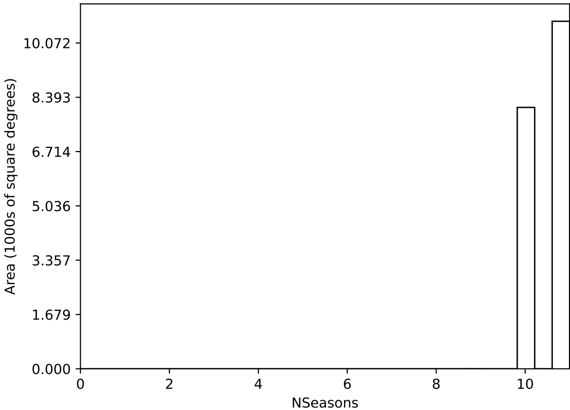
internal_u_expt60_nscale1.1v3.4_10yrs WFD all bands: NSeasons
