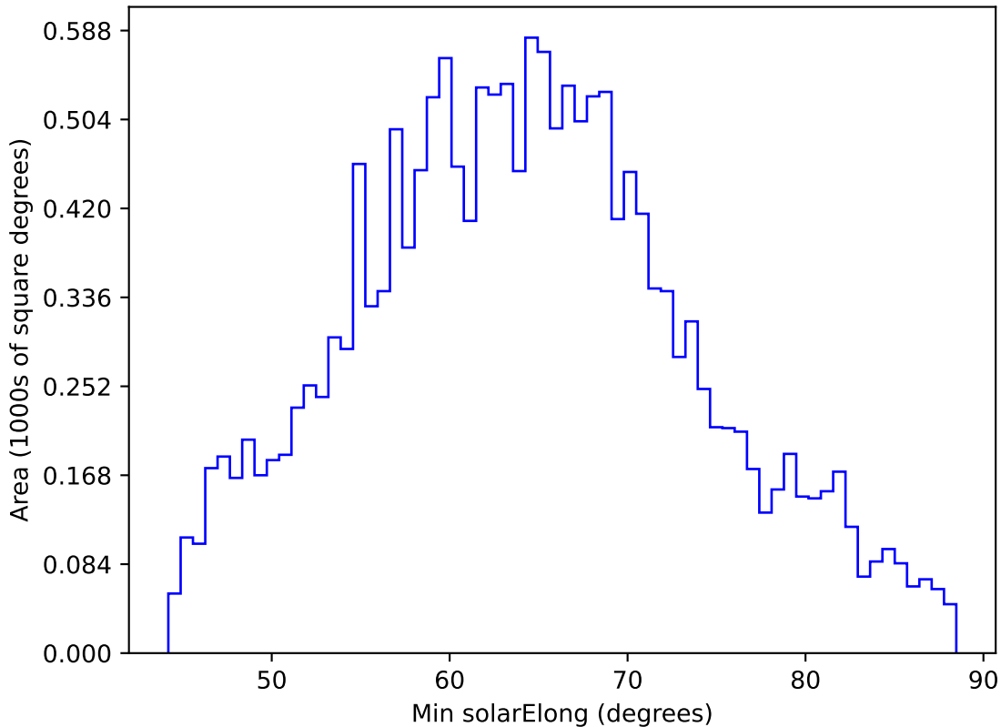
internal_u_expt60_nscale1.1v3.4_10yrs WFD y band: Min solarElong
