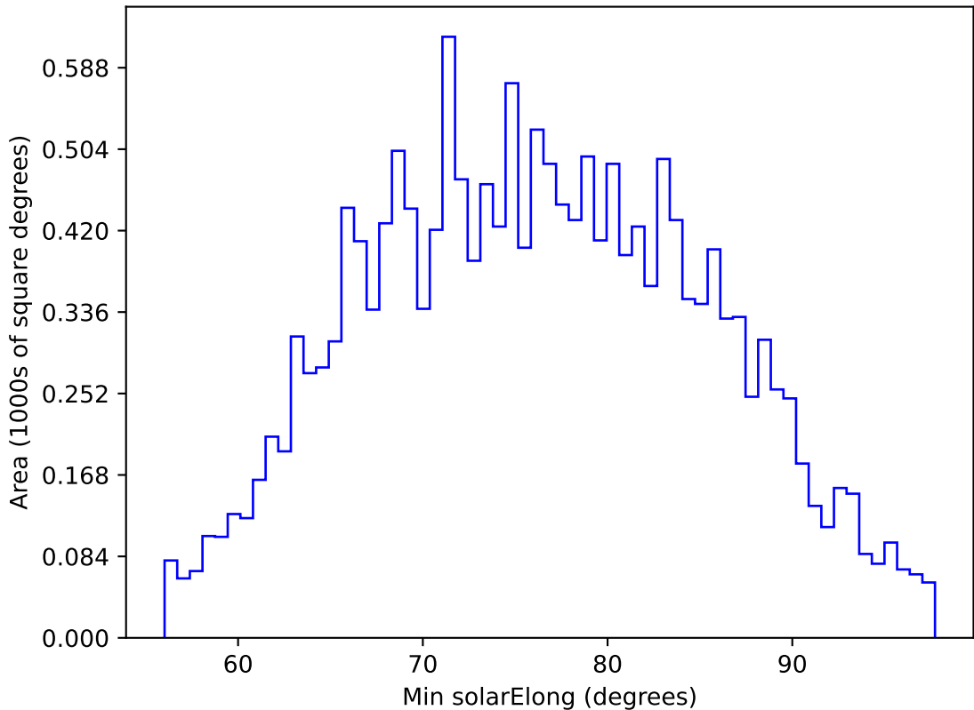
internal_u_expt60_nscale1.1v3.4_10yrs WFD g band: Min solarElong
