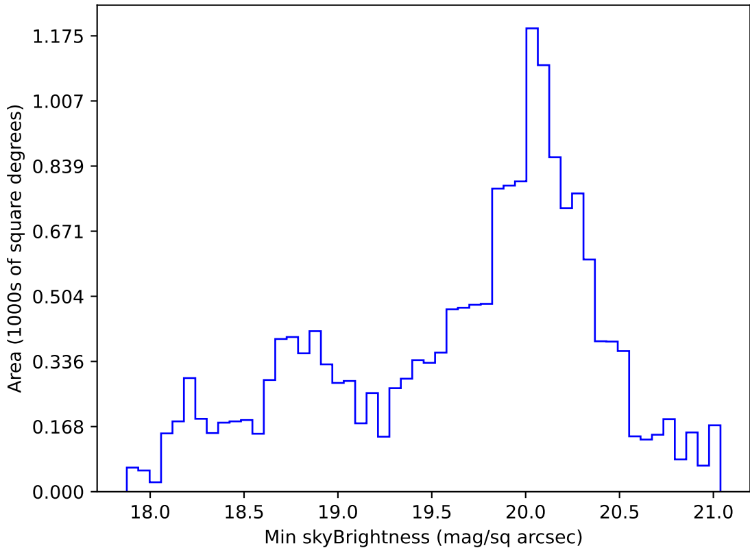
internal_u_expt60_nscale1.1v3.4_10yrs WFD g band: Min skyBrightness
