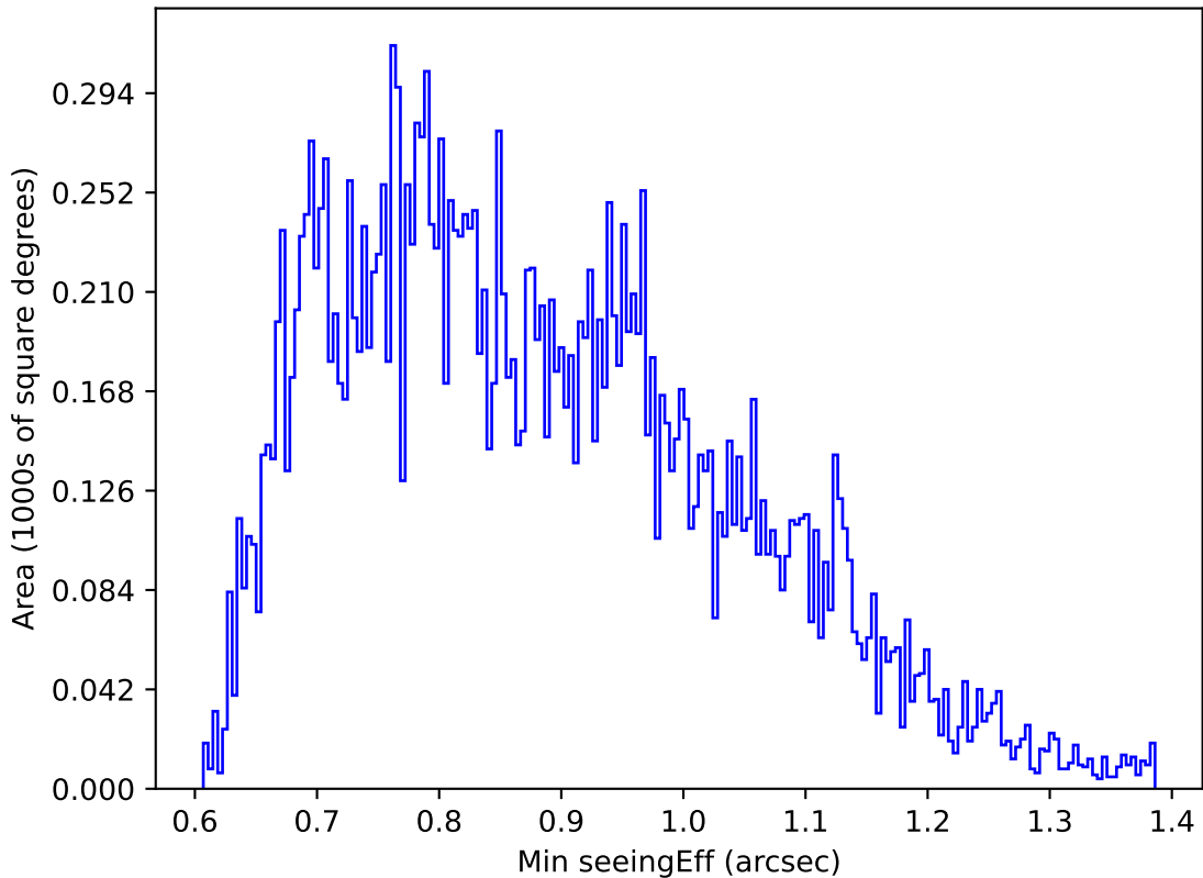
internal_u_expt60_nscale1.1v3.4_10yrs Yr 1 u band: Min seeingEff
