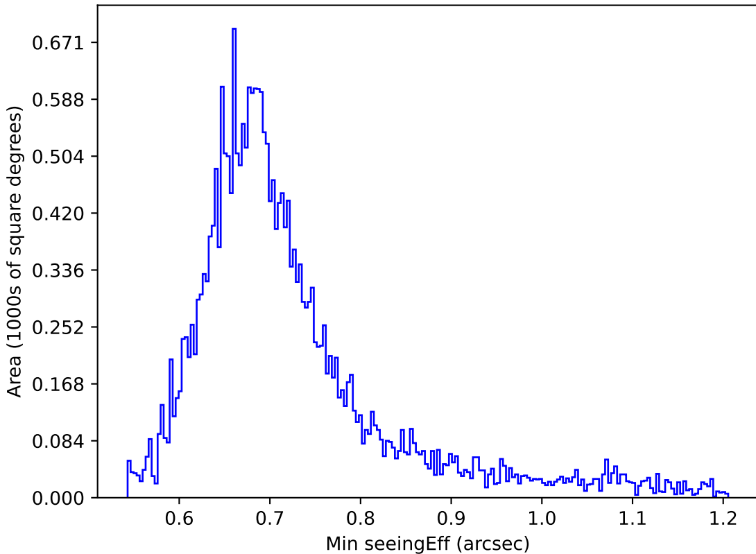
internal_u_expt60_nscale1.1v3.4_10yrs Yr 1 r band: Min seeingEff
