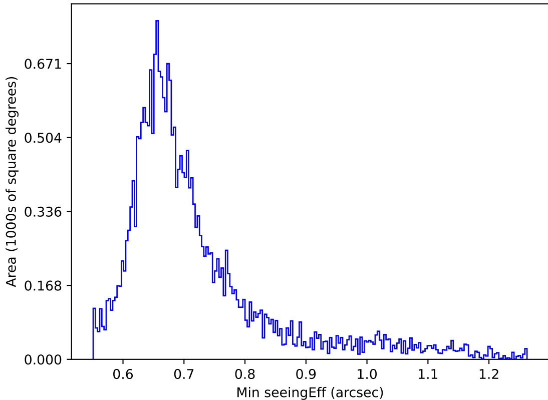
internal_u_expt60_nscale1.1v3.4_10yrs Yr 1 i band: Min seeingEff
