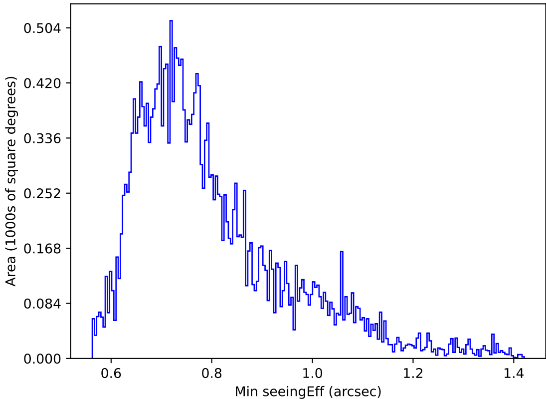
internal_u_expt60_nscale1.1v3.4_10yrs Yr 1 g band: Min seeingEff
