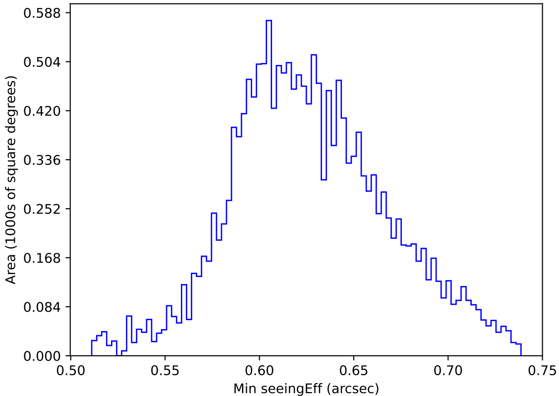
internal_u_expt60_nscale1.1v3.4_10yrs WFD y band: Min seeingEff
