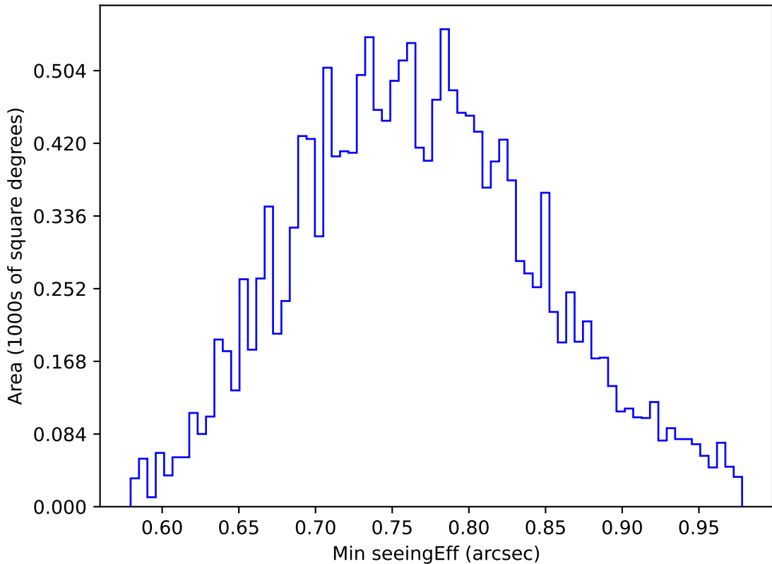
internal_u_expt60_nscale1.1v3.4_10yrs WFD u band: Min seeingEff
