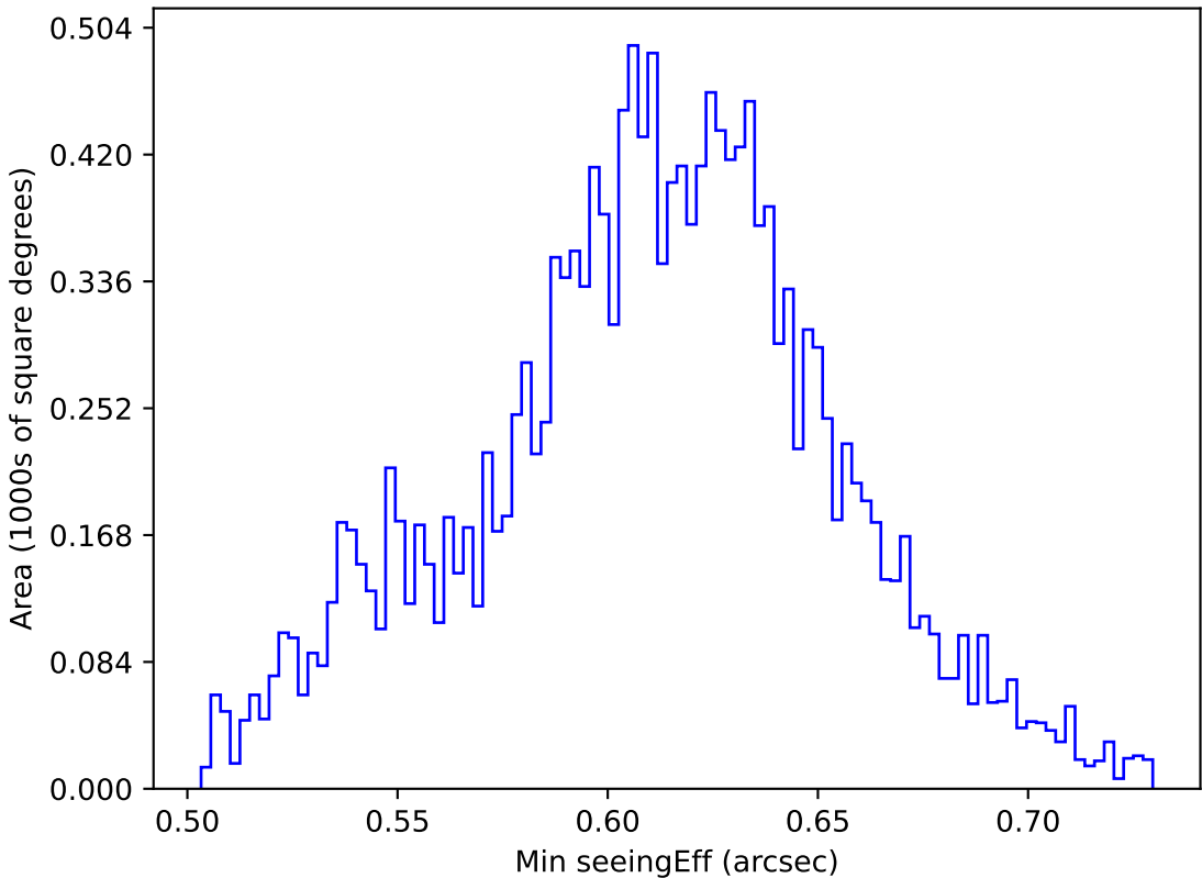
internal_u_expt60_nscale1.1v3.4_10yrs WFD r band: Min seeingEff
