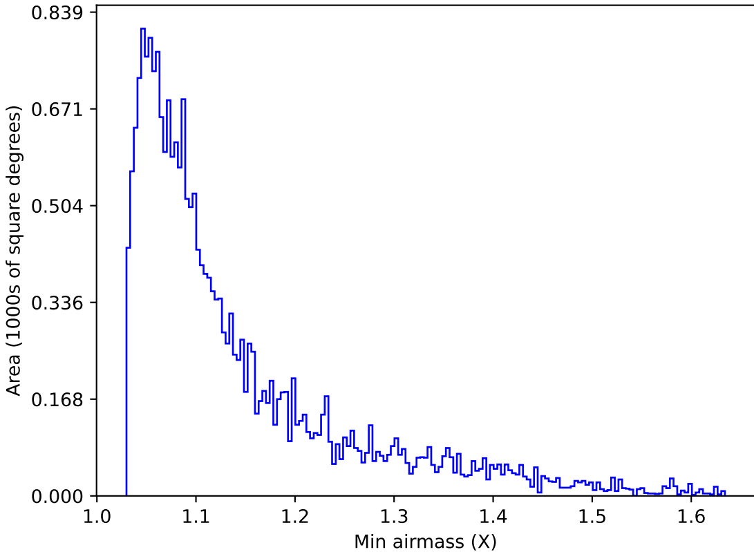
internal_u_expt60_nscale1.1v3.4_10yrs Yr 1 u band: Min airmass
